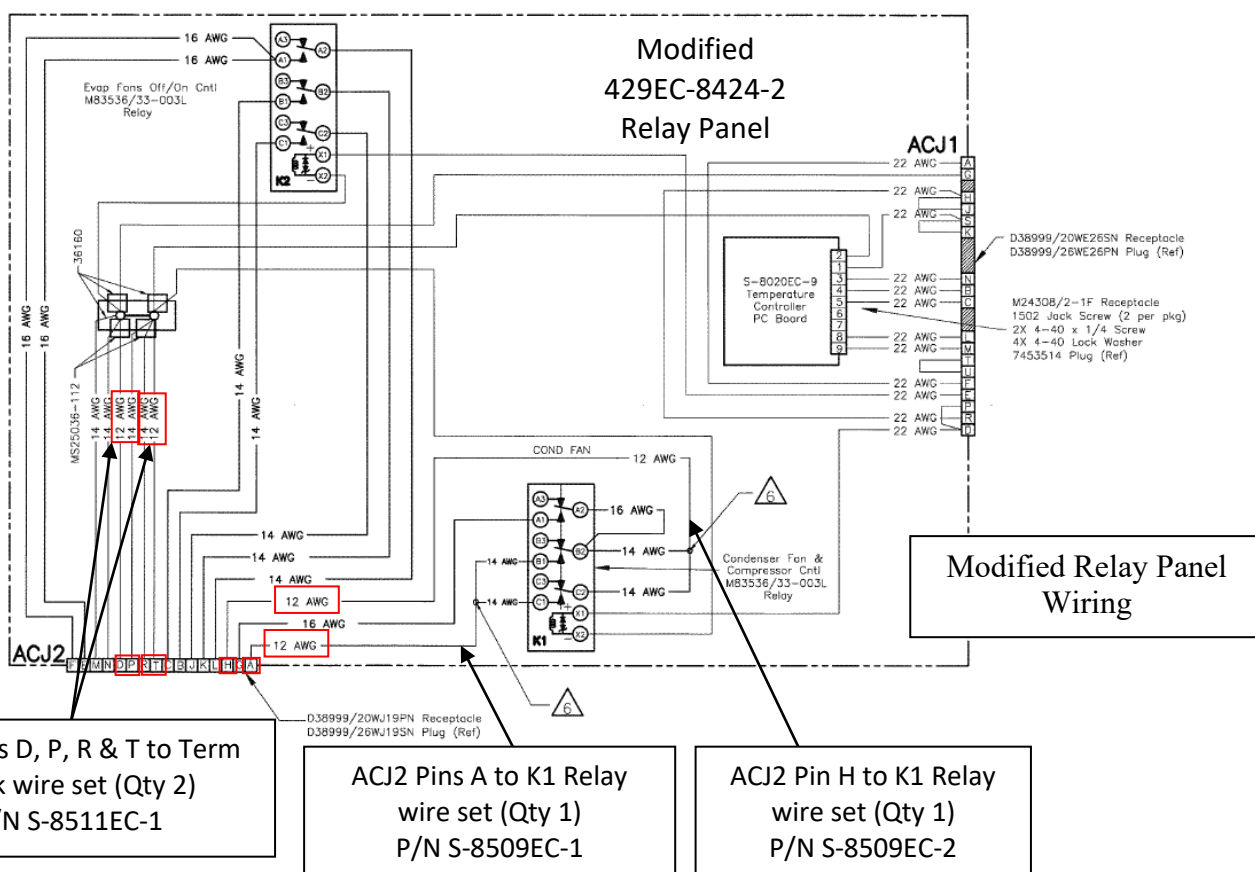
Figure 6. 429EC-8424EC-2 Relay Panel Box Wiring, existing and modified
