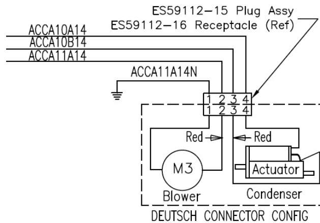
Figure 3: Deutsch Connector Configuration
