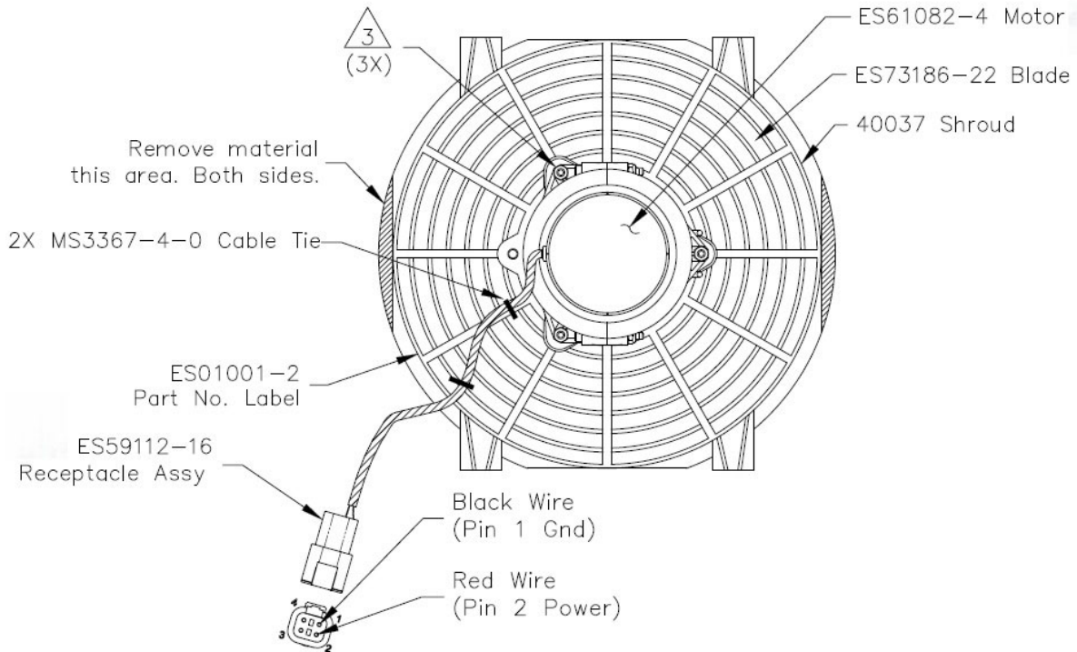
Figure 2: Blower Assembly ES73192-4
