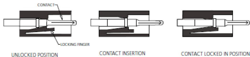
Figure 4: Contact Insertion
