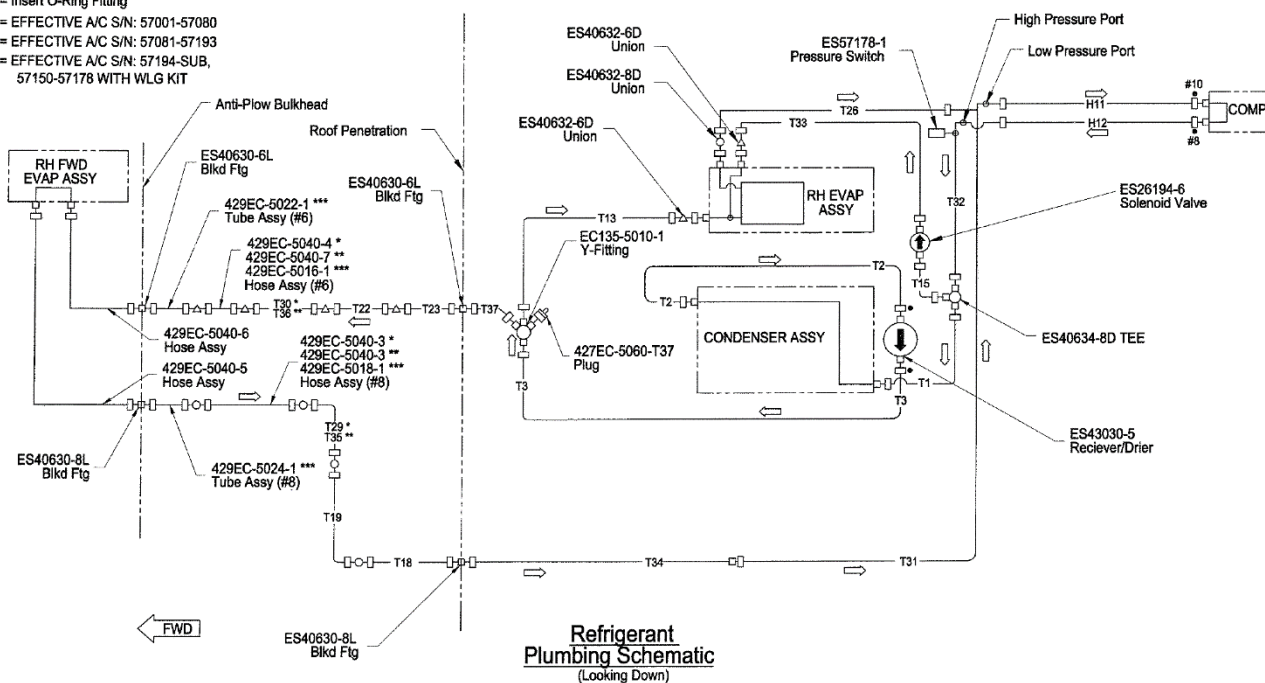
Figure 3: Air Conditioner Plumbing (Single Fwd/Aft Evaporators)
