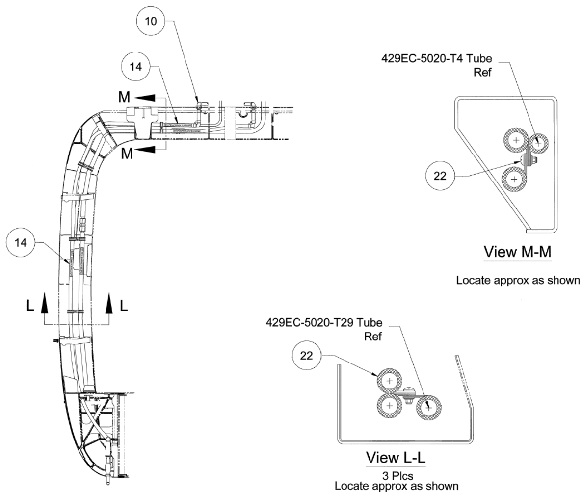
Figure 23: LH Aft Evaporator Drain Line Installation View Looking Fwd, LH Side
