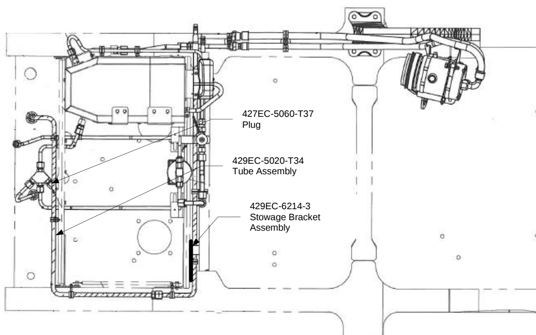
Figure 11: RH Aft Evaporator – View Looking Down (Condenser Assembly not shown for clarity)
