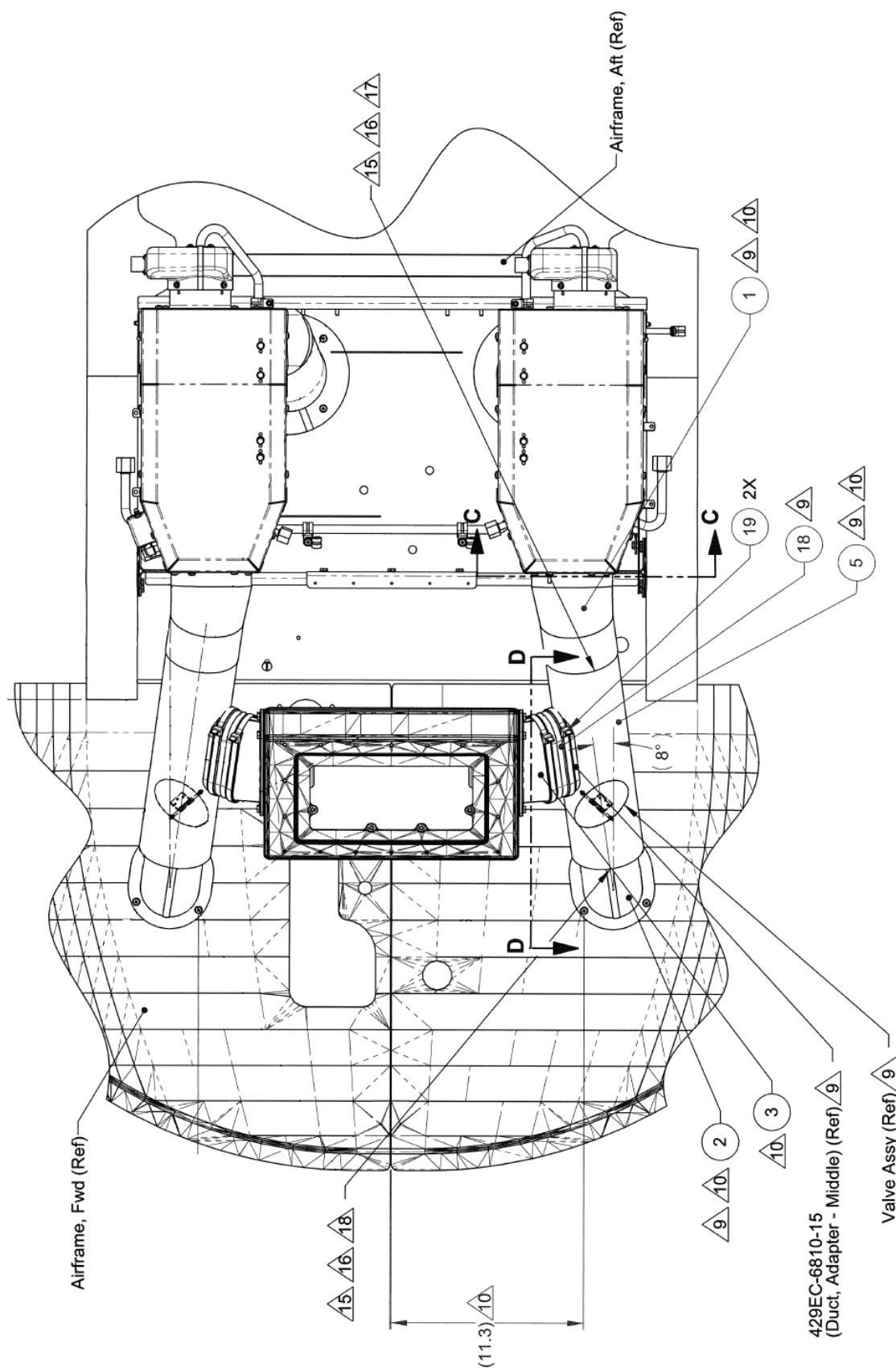
Figure 21: LH Aft Evaporator Installation – View Looking Down
