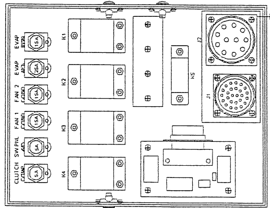
Figure 2 Air Conditioner Control Panel (Located in center console)
